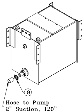
Suction Line
