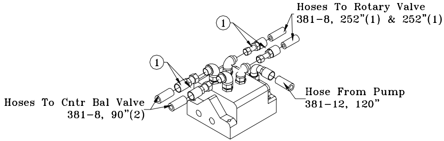
Valve Bank
